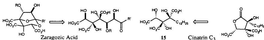
Figure 2. Structures of cinatrin C 3 ( 13 ) and cinatrin C 1 ( 14 ) as assigned by Itazaki (ref. 3) and their common precursor ( 15 ).
